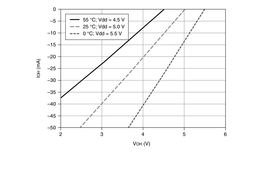
Figure 3. PFI <0..15>/P0.<0..15>: I oh versus V oh
